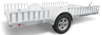
Model 1694. Featherlite's open trailer Model 1694 offers side kits as a standard feature. These are removable and also serve as the trailer's ramp. The 1694 also features standard tie down rings to further secure your motorcycle. Length options are 10' or 12' with a width of 6'6".
